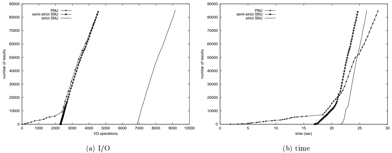
Figure 7: Spatial join ST \bowtie RR: Number of results as a function of I/O and time
