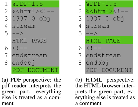
Figure 1: Structure of the janiform PDfF format
