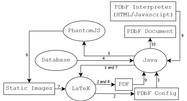
Figure 2: Compilation steps of the PDfF compiler framework
